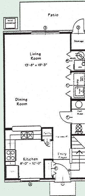
Three Bedroom Townhouse 1 1/2 bath Total 1,058 S.F.
