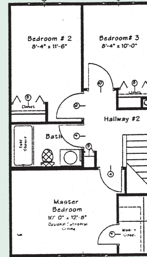
Three Bedroom Townhouse 1 1/2 bath Total 1,058 S.F.
